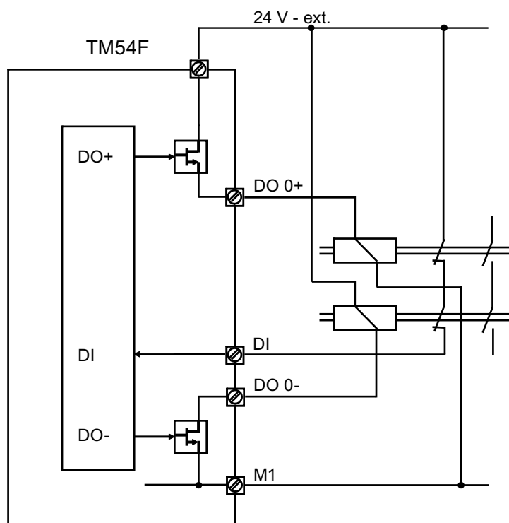
Figure 7-7 F-DO circuit, test stop mode 2
