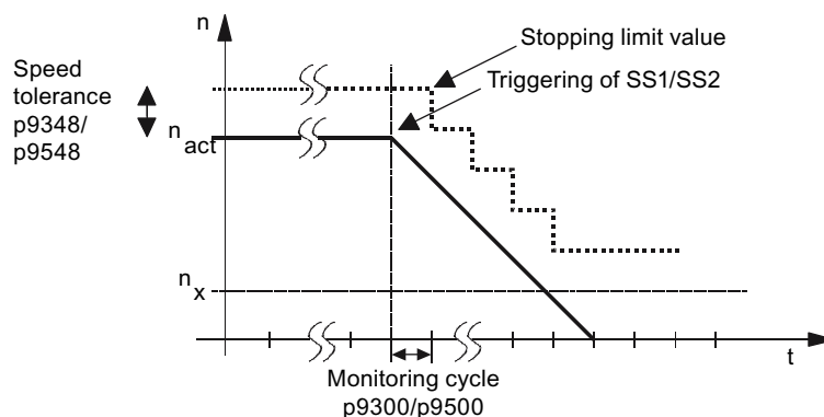
Figure 5-8 Characteristics of the shutdown limit for SBR
