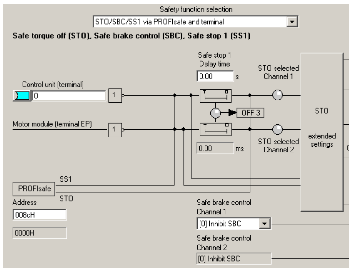
Figure 7-24 STARTER screen section from Safety Integrated: Setting the PROFIsafe address (example)
