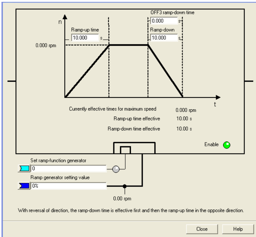
Figure 7-2 Ramp-function generator ramp
