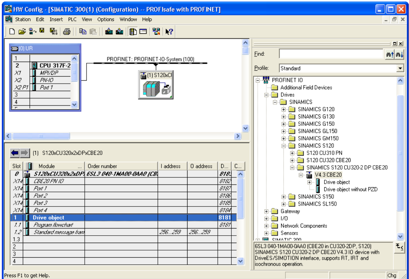
Figure 7-25 Configuration of the PROFINET connection in HW Config
