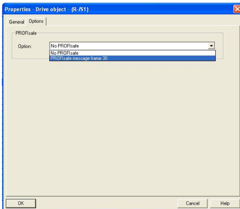
Figure 7-26 Drive object option "PROFIsafe telegram"
