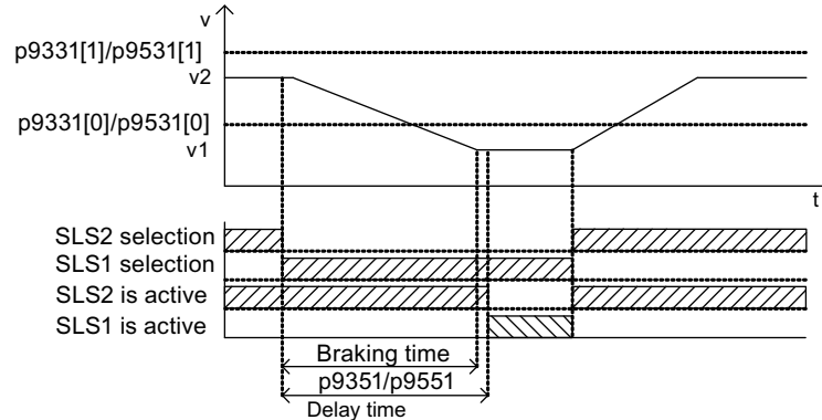
Figure 5-5 Delay time SLS speed limit value
