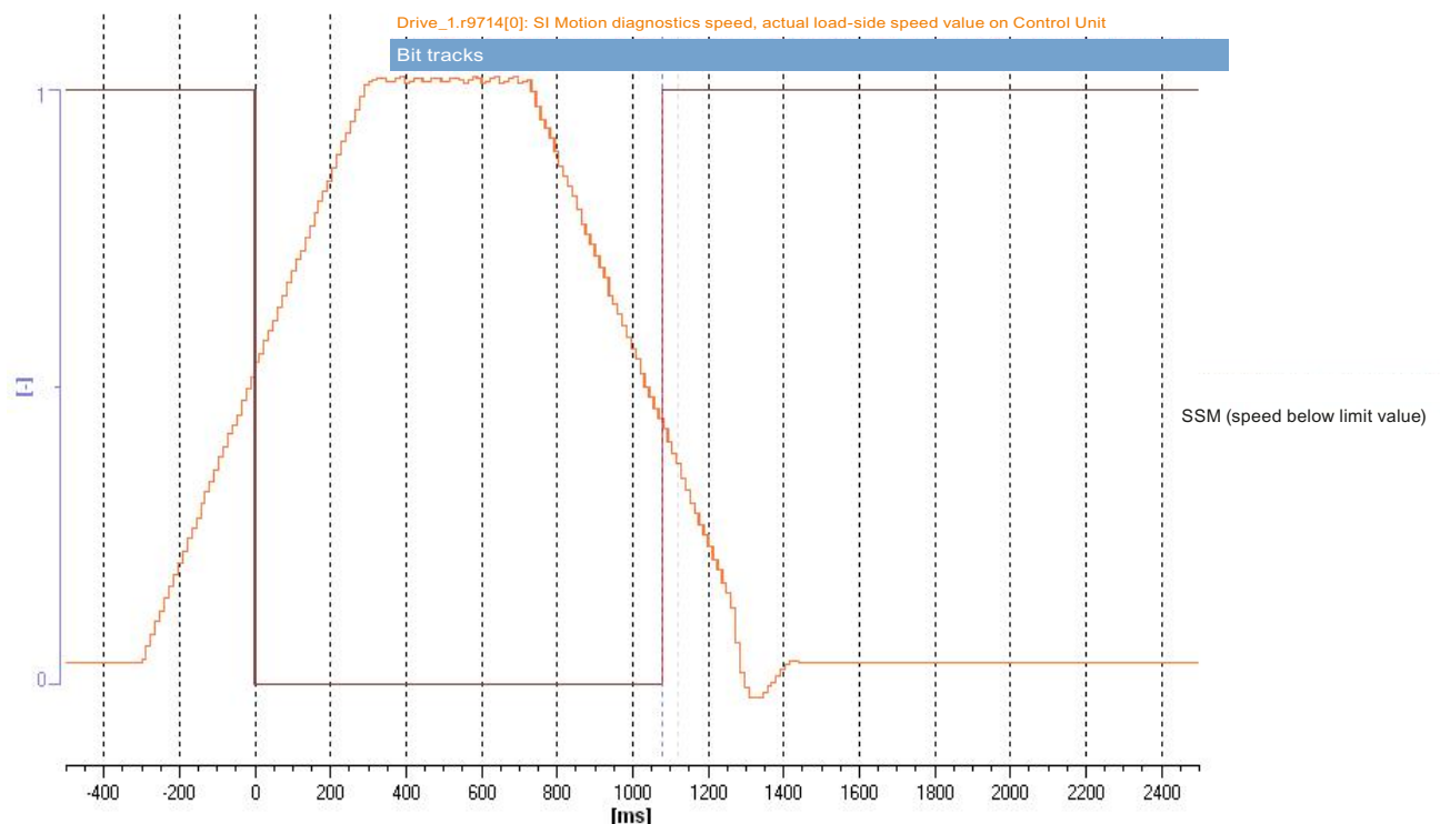
Figure 9-8 Example Trace SSM (with hysteresis)
