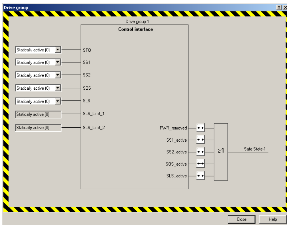
Figure 7-11 Screen, drive group
