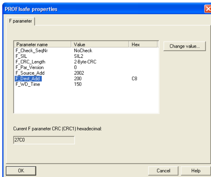
Figure 7-23 Setting the F parameters
