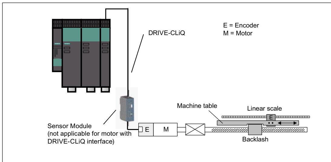
Figure 5-11 Example of an S120 single-encoder system
