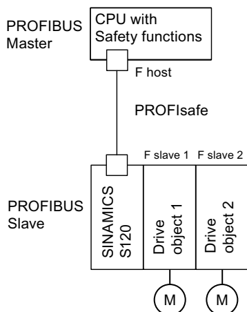
Figure 7-12 Example of a PROFIsafe topology
