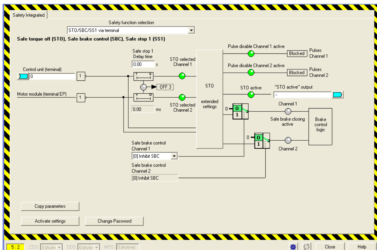
Figure 7-32 STO/SBC/SS1 via terminals
