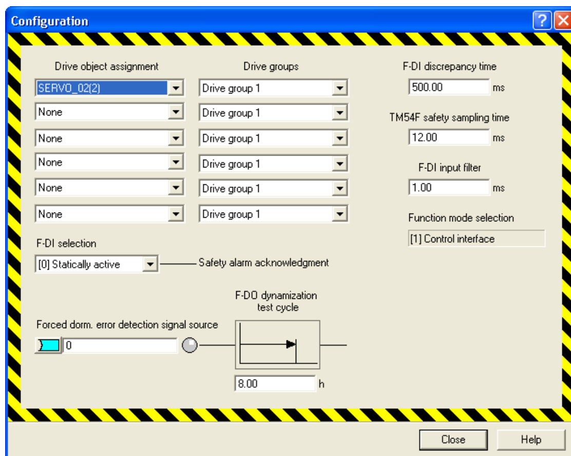
Figure 7-5 TM54F configuration
