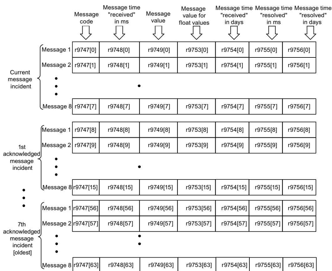
Figure 5-10 Structure of the message buffer
