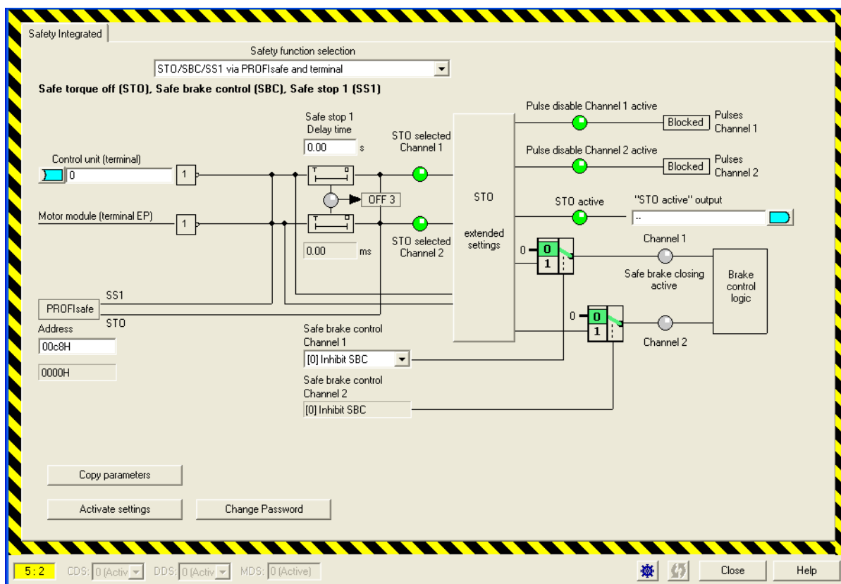
Figure 7-34 STO/SBC/SS1 via PROFIsafe and terminal
