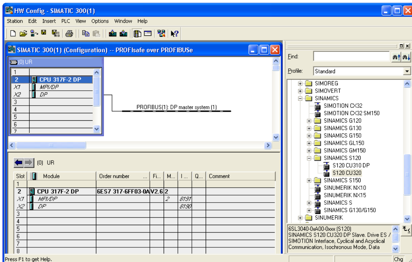
Figure 7-20 Selecting a drive
