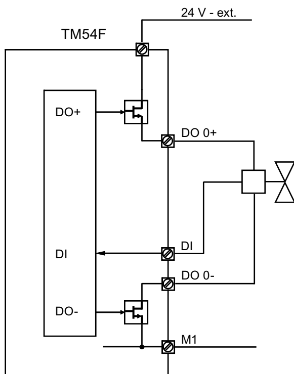
Figure 7-8 F-DO circuit, test stop mode 3
