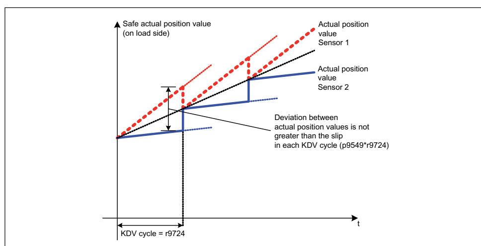
Figure 5-14 Example diagram of actual value synchronization
