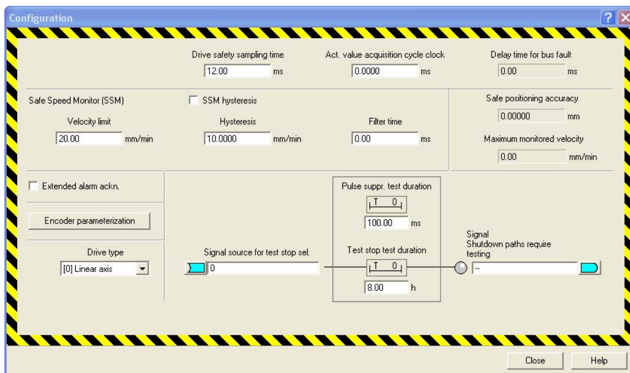
Figure 7-36 Safety configuration: Drive
