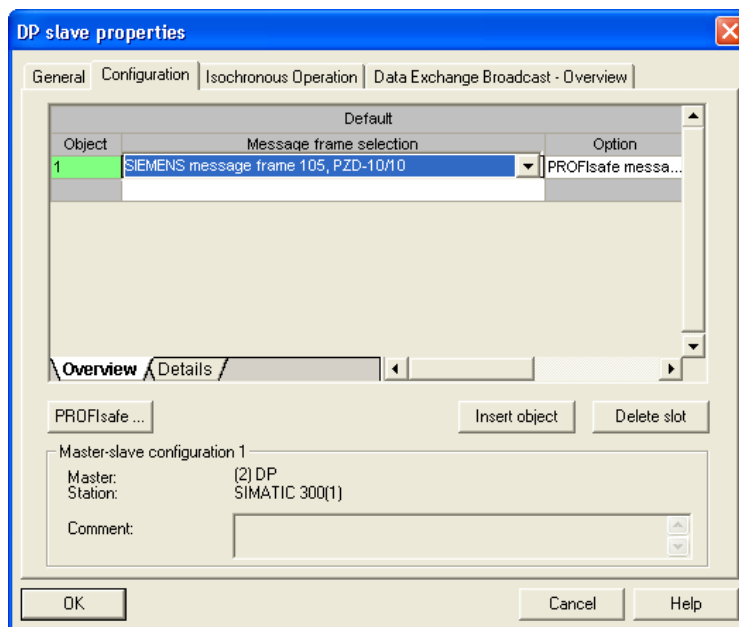
Figure 7-22 PROFIBUS DP slave properties
