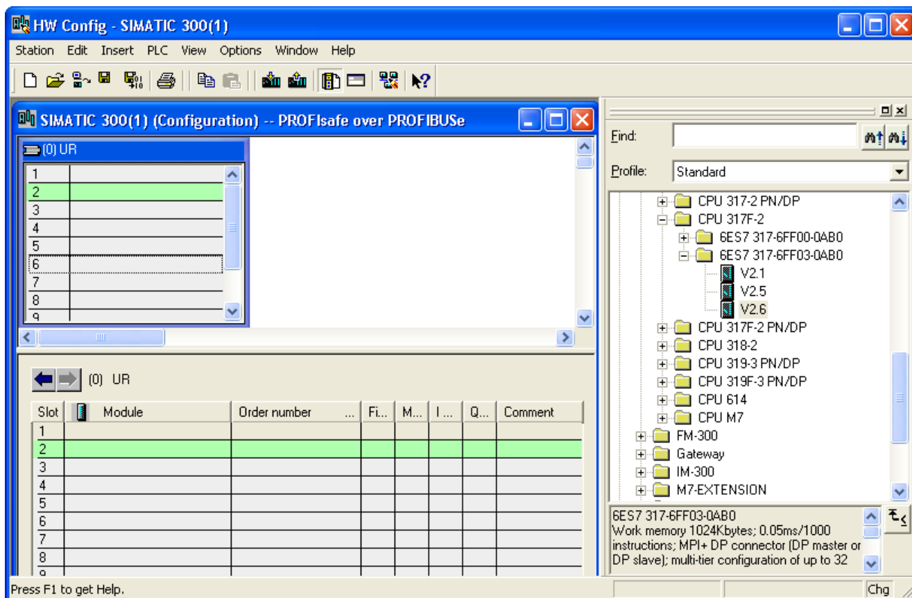
Figure 7-17 Creating an F host (master)
