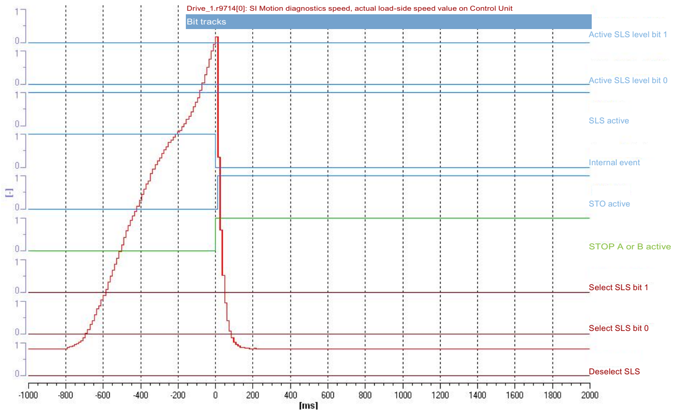
Figure 9-10 Example trace SLS without encoder with STOP A
