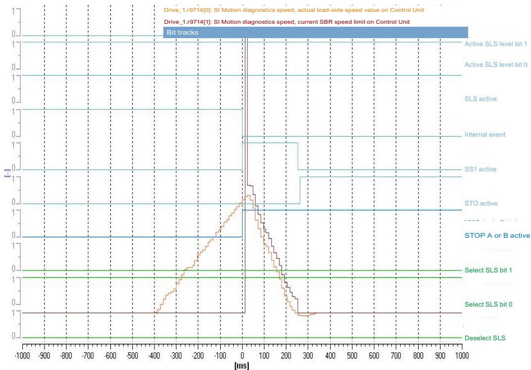
Figure 9-5 Example trace: SLS with STOP B
