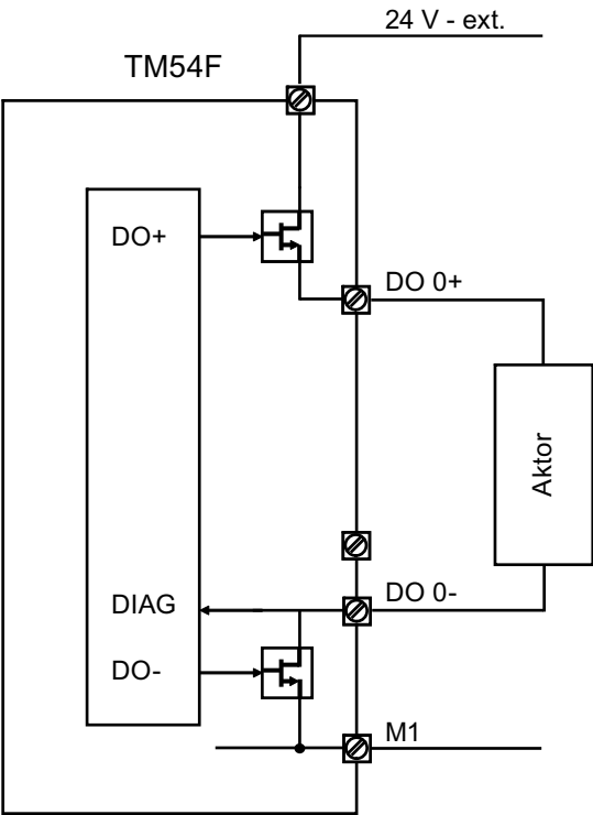
Figure 7-6 F-DO circuit, test stop mode 1
