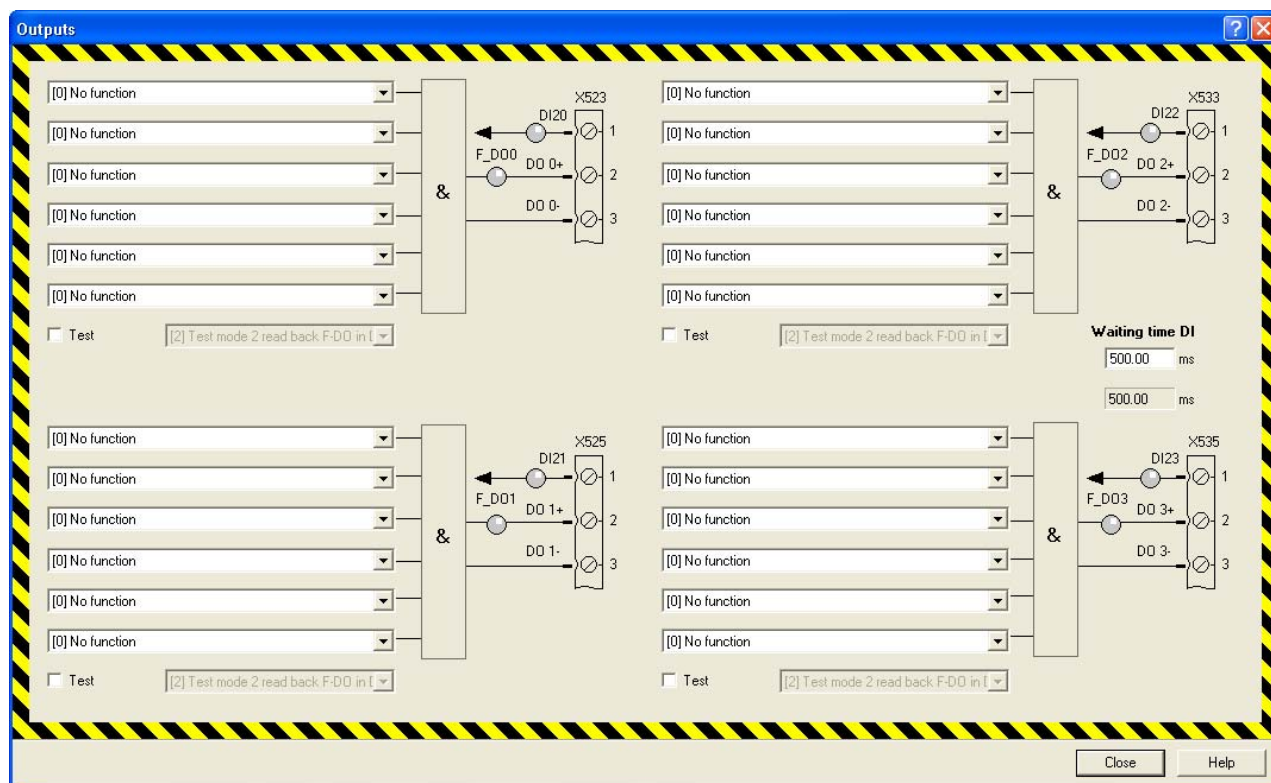
Figure 7-10 Outputs screen
