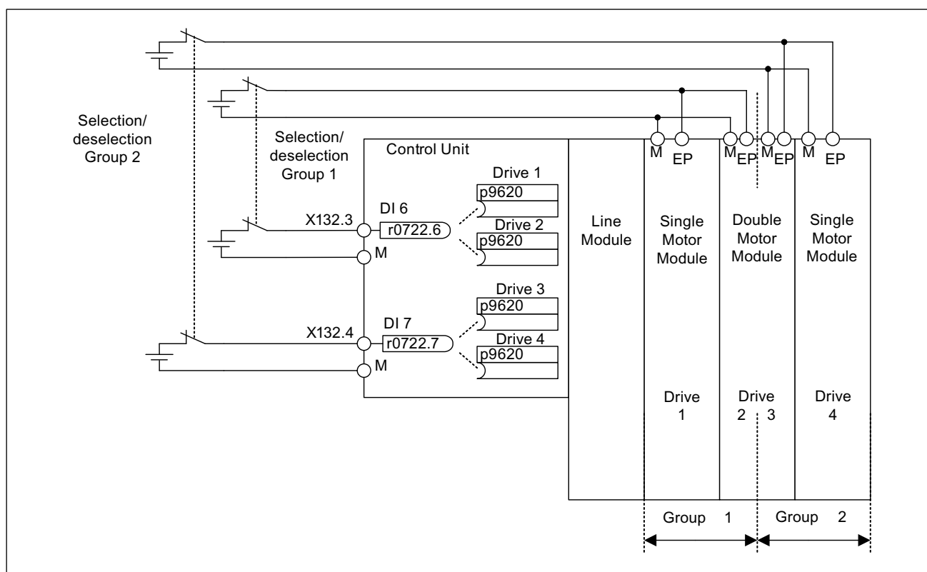
Figure 6-2 Example: Grouping terminals with Motor Modules booksize and CU320-2 DP
