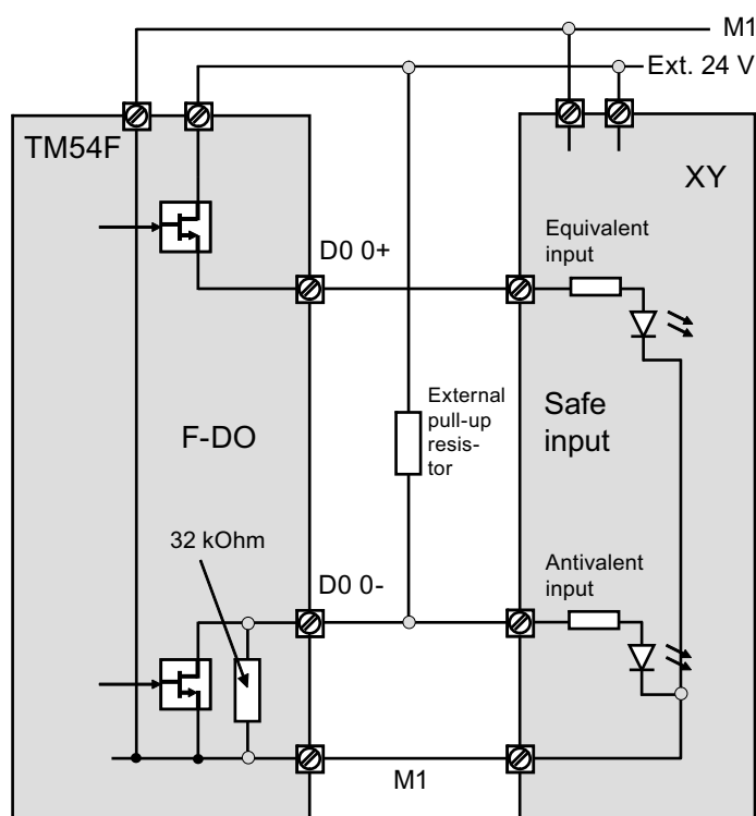
Figure 8-1 TM54F F-DO at equivalent/antivalent safe input on safety switching device (e.g. safety PLC)
