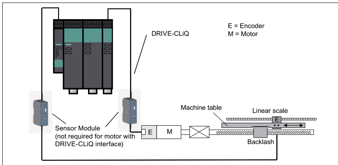
Figure 5-12 Example of an S120 two-encoder system on a linear axis via a ballscrew
