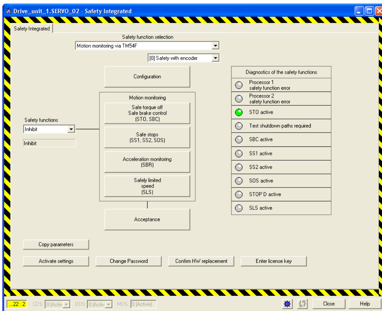
Figure 7-35 Safety Integrated commissioning of a linear/rotary axis
