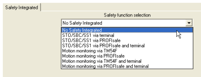
Figure 7-3 Safety Integrated selection
