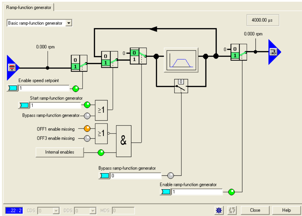
Figure 7-1 Ramp-function generator
