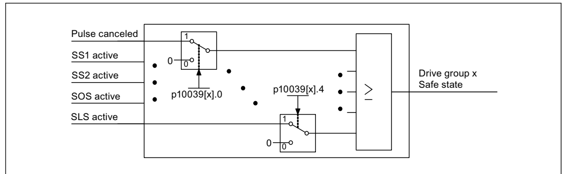
Figure 6-4 Safe state selection
