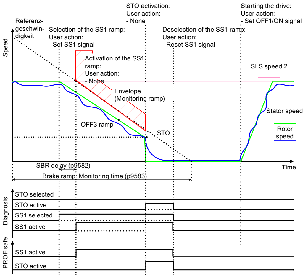
Figure 5-9 Safe Brake Ramp without encoder
