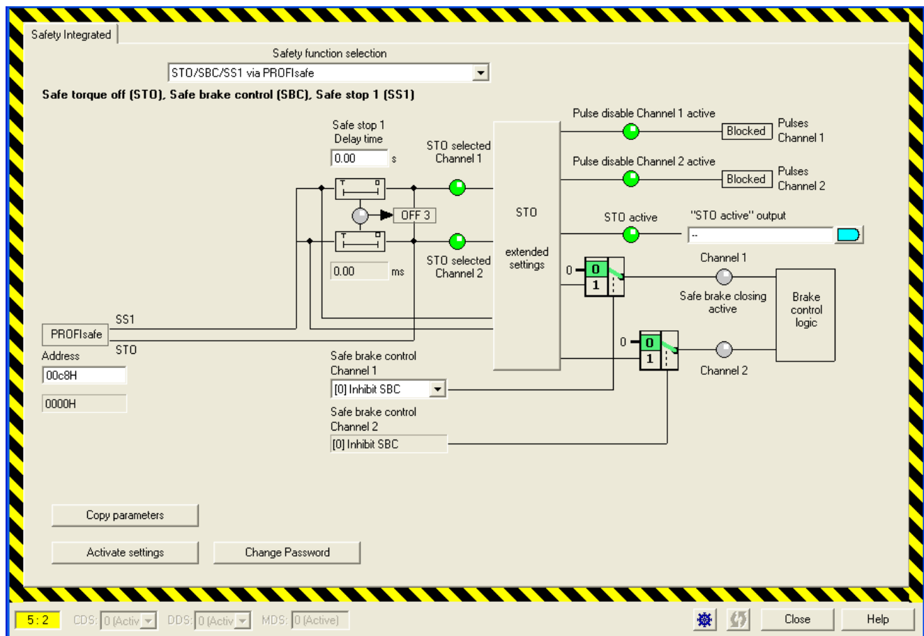
Figure 7-33 STO/SBC/SS1 via PROFIsafe
