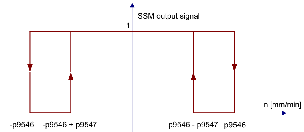
Figure 5-7 Safe output signal for SSM with hysteresis
