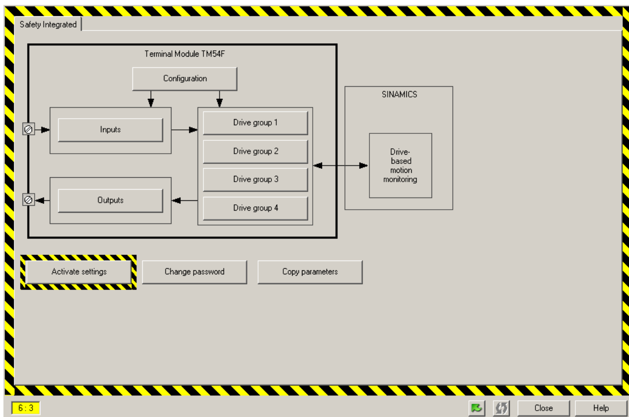
Figure 7-4 Configuration start screen TM54F
