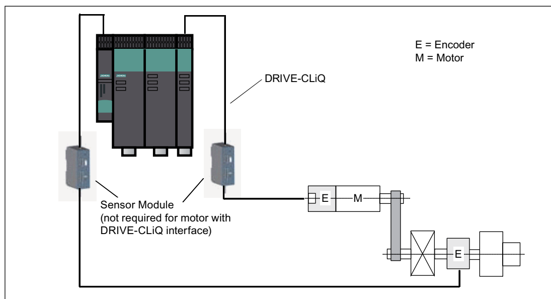
Figure 5-13 Example of an S120 two-encoder system on a rotary axis
