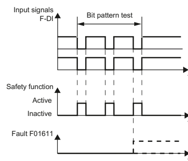
Figure 6-3 Inverter response to a bit pattern test
