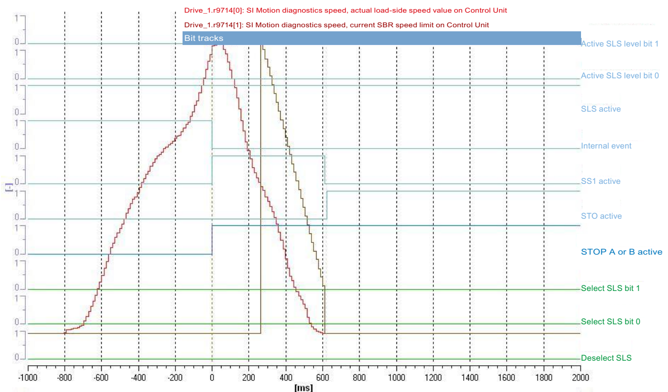
Figure 9-11 Example trace SLS without encoder with STOP B
