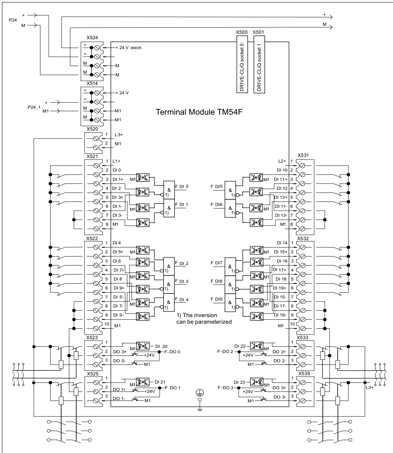
Figure 5-15 Example of the TM54F wiring
