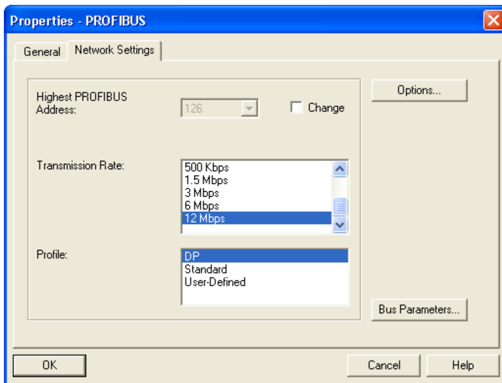
Figure 7-19 Setting the PROFIBUS profile
