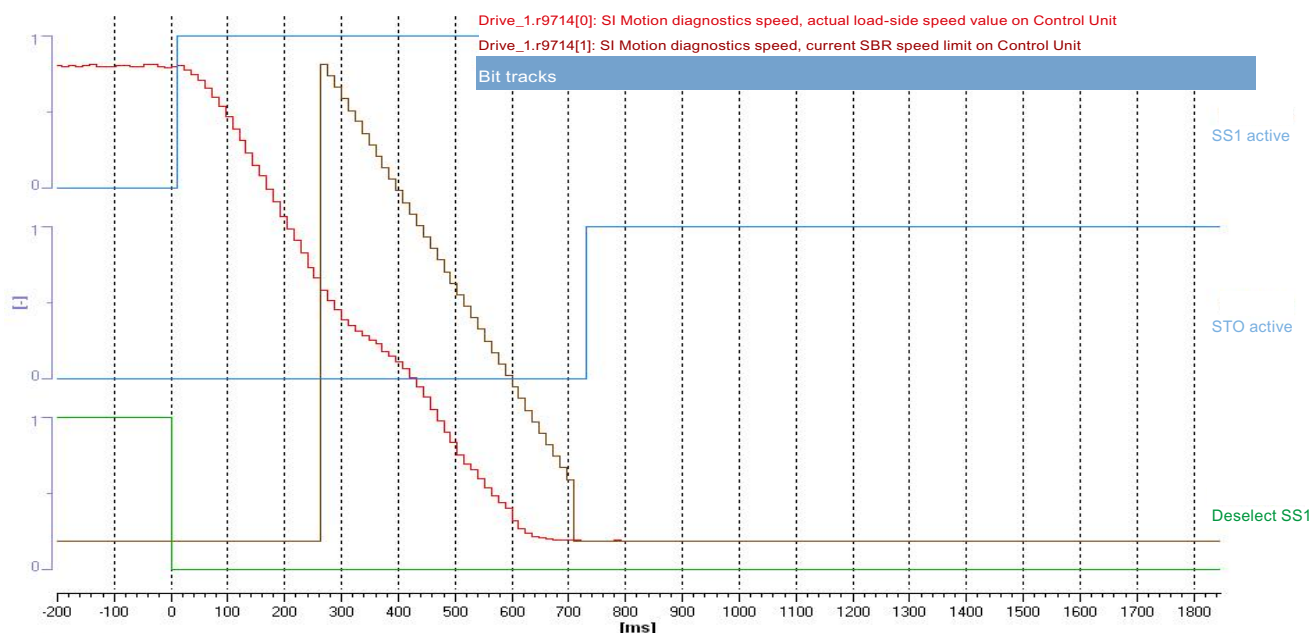
Figure 9-9 Example Trace SS1 without encoder
