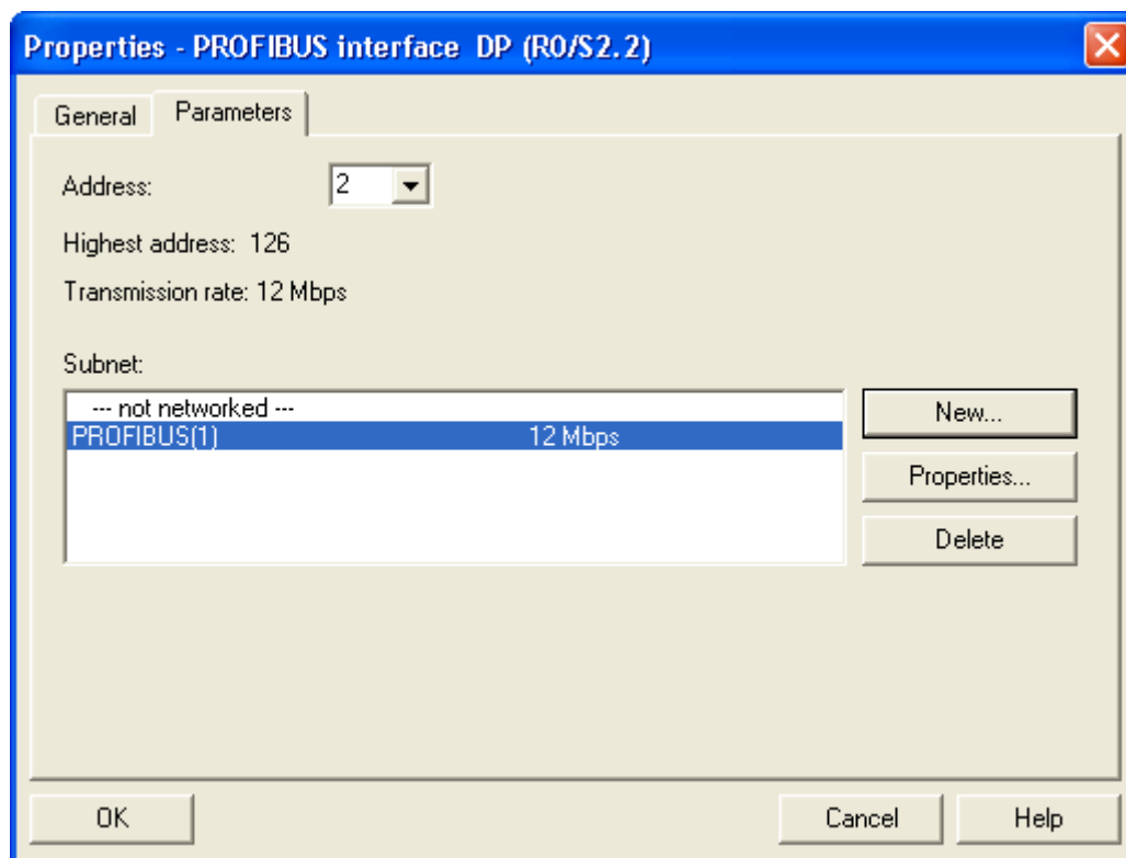
Figure 7-18 Setting the PROFIBUS interface
