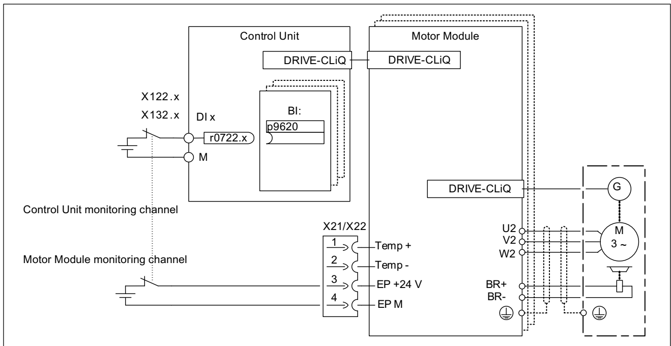
Figure 6-1 Example: Terminals for "Safe Torque Off", example for Motor Modules booksize and CU320-2 DP
