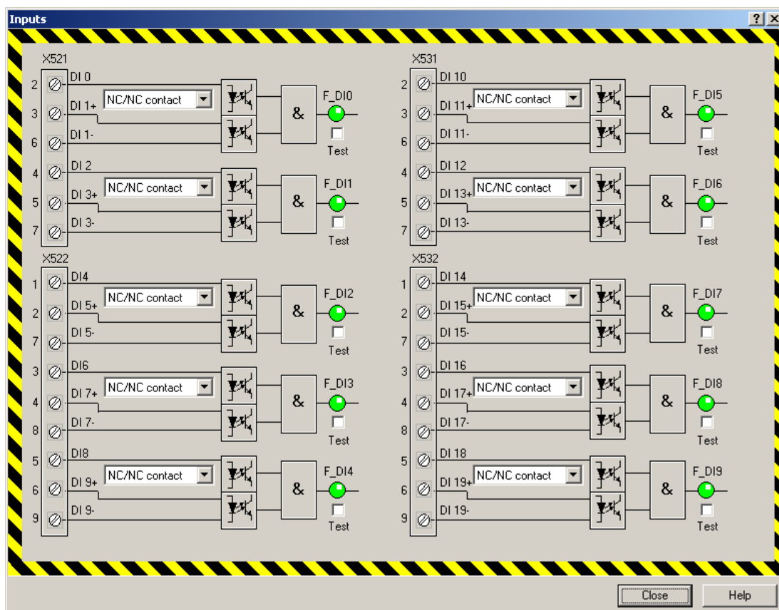
Figure 7-9 Inputs screen
