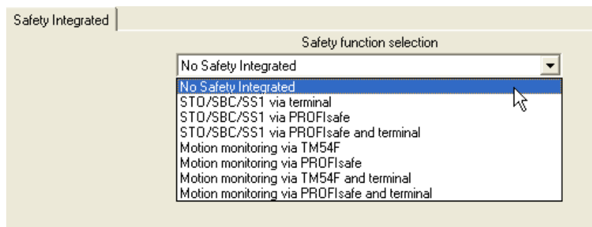
Figure 7-31 Safety_Integrated_Auswahl
