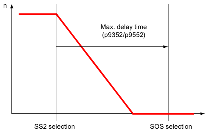
Figure 5-3 Sequence with SS2 selection
